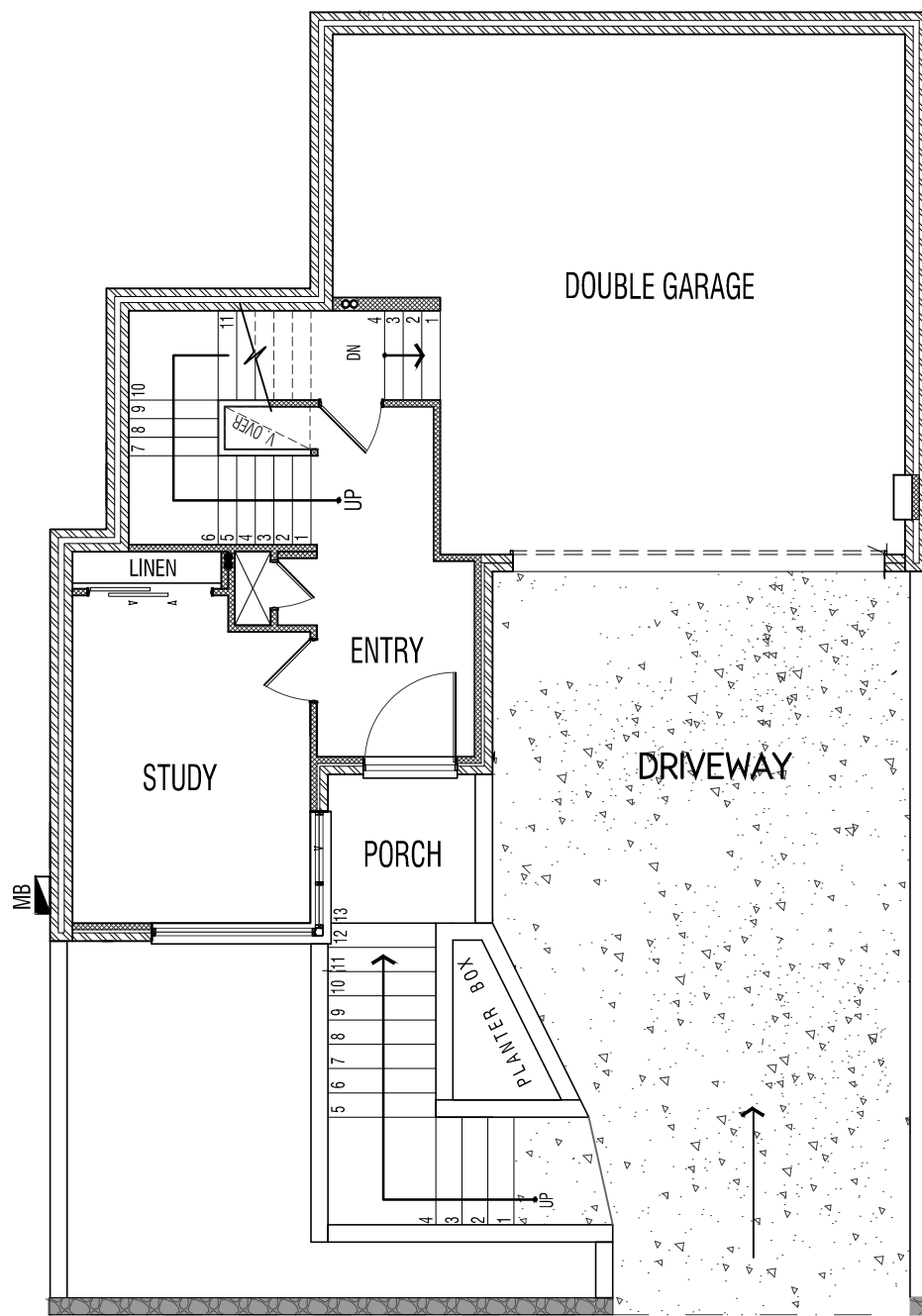
Basement Floor
