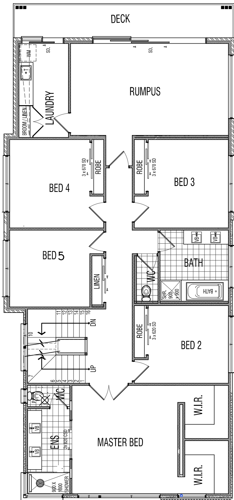
Ground Floor
