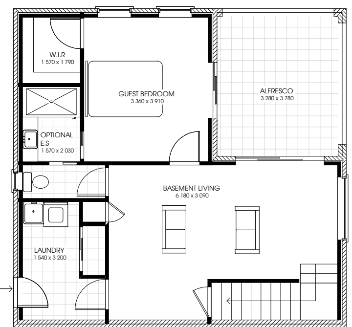
BASEMENT FLOOR
