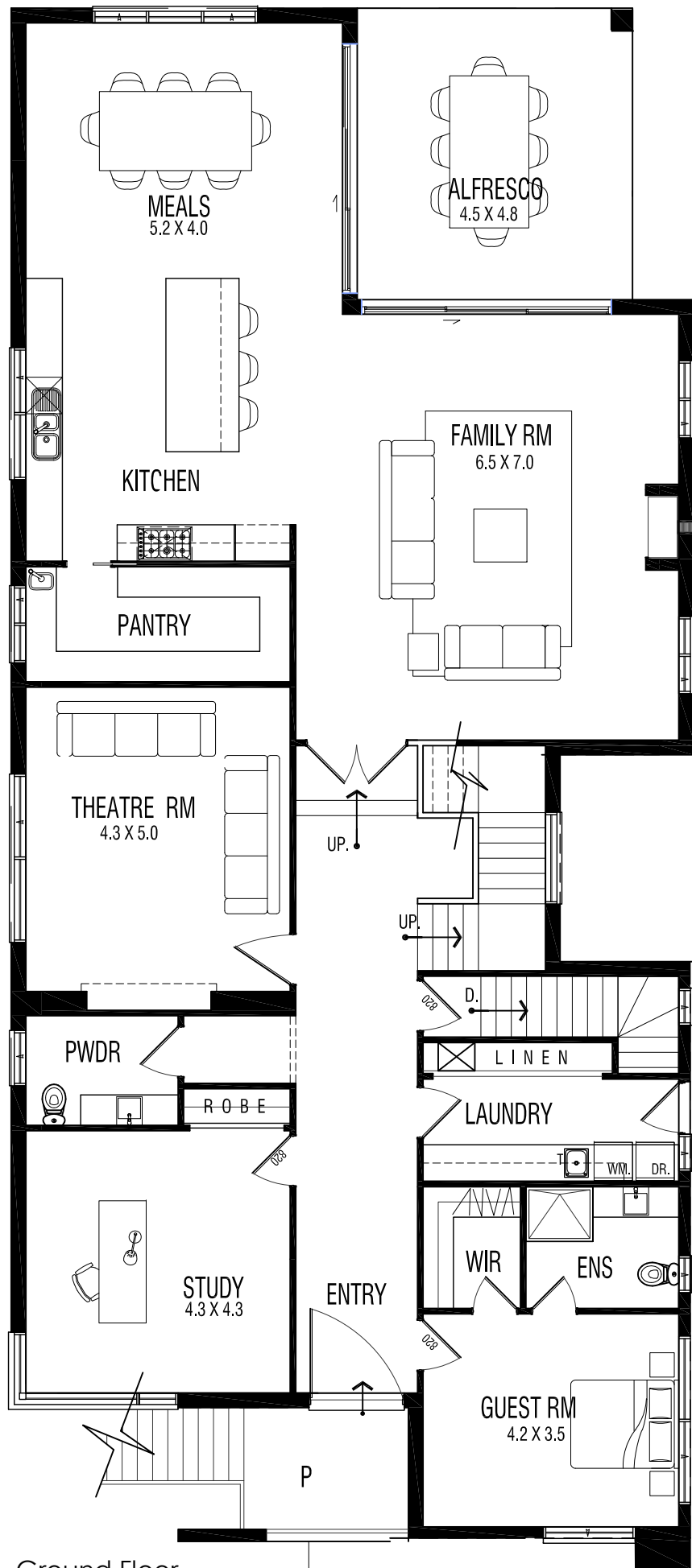
Ground Floor
