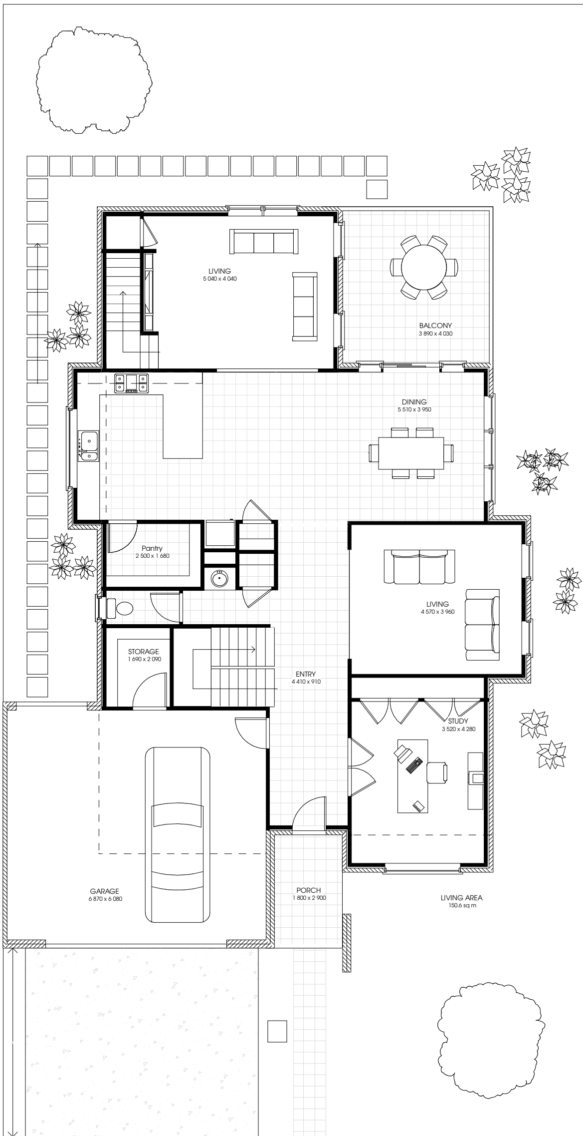
GROUND FLOOR/MAIN FLOOR
